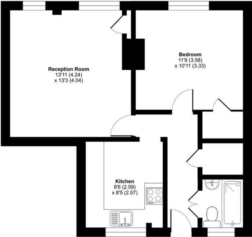
FIRST FLOOR
